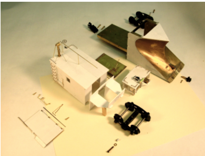
ABOVE: Exploded view showing major parts before assembly.
